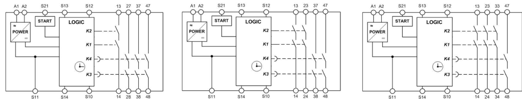
Fig. 1 Block diagram: SR4C (1nd/3d); SR4C (2nd/2d); SR4C (3nd/1d)
