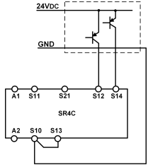
Fig. 5: Two-channel emergency stop with pnp-outputs/OSSD-outputs with short circuit monitoring. (up to category 4, PL e)
